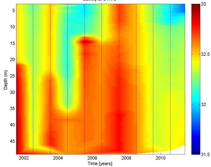
Salinity at UTN-5
