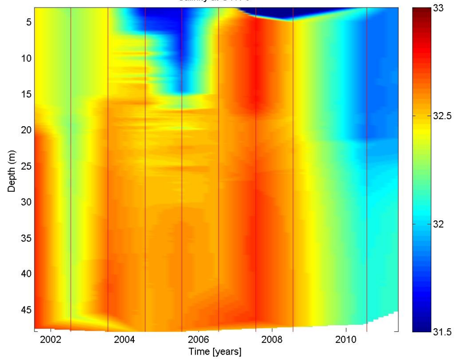
Salinity at UTN-6
