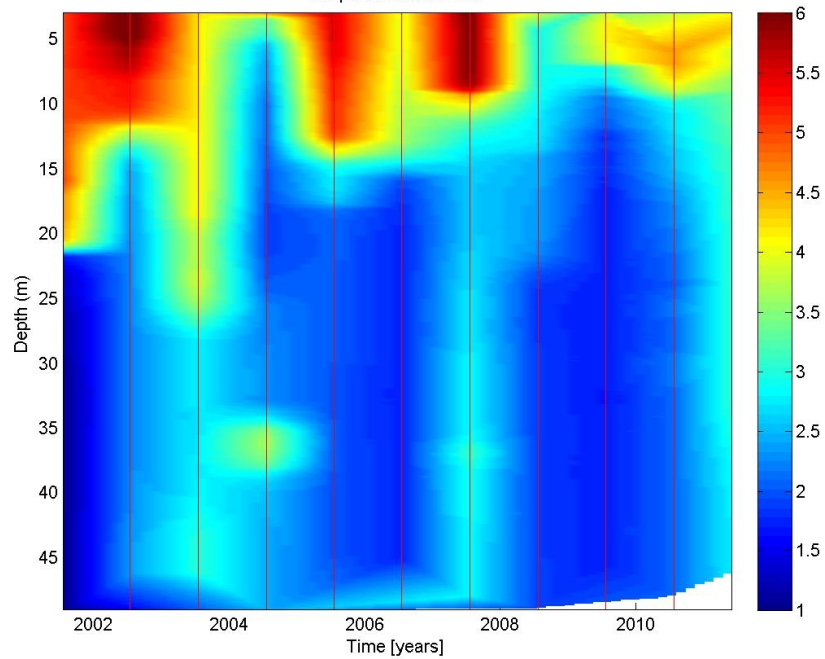
Temperature at UTN-5
