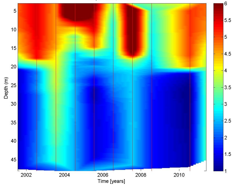
Temperature at UTN-6
